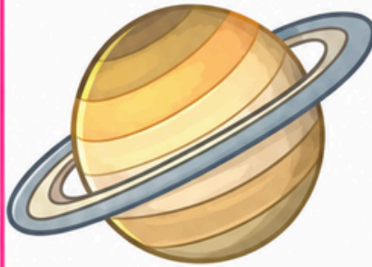
Saturn
