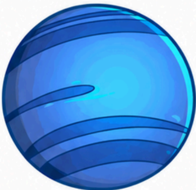
Neptune
