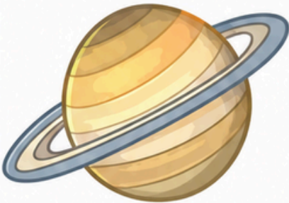
Saturn
