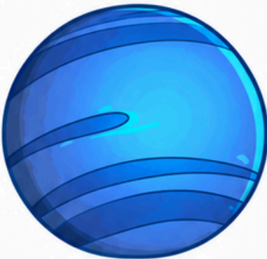
Neptune
