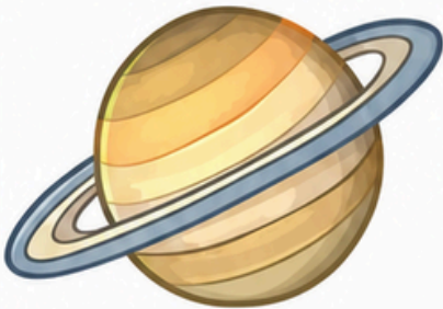
Saturn
