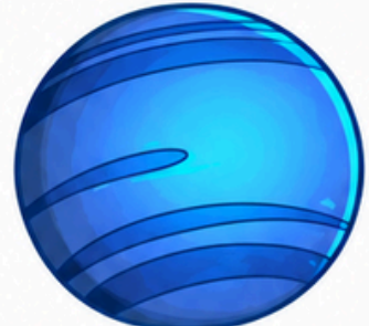
Neptune
