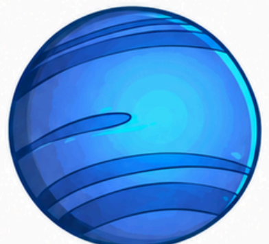
Neptune
