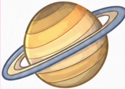
Saturn
